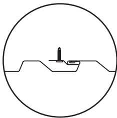
WAVE FIXED SEAM ENGAGEMENT
