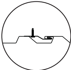
WAVE FLOATING SEAM ENGAGEMENT
